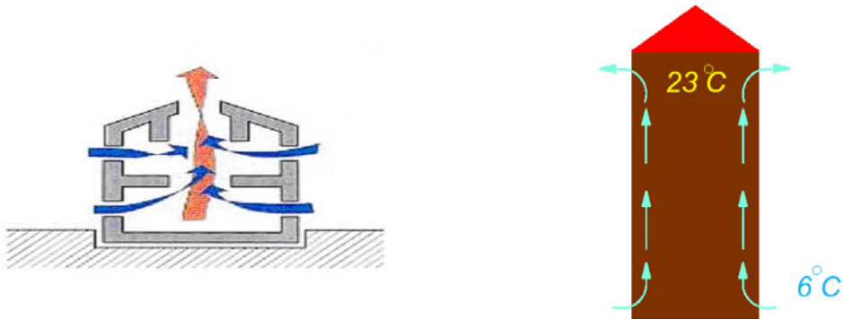
Natural Ventilation: Stack Effect
