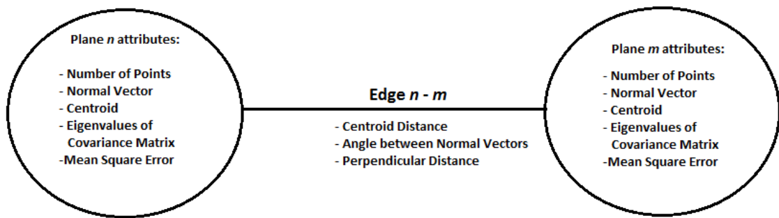
Figure 3.5: Information stored in each node and each edge of the graph
