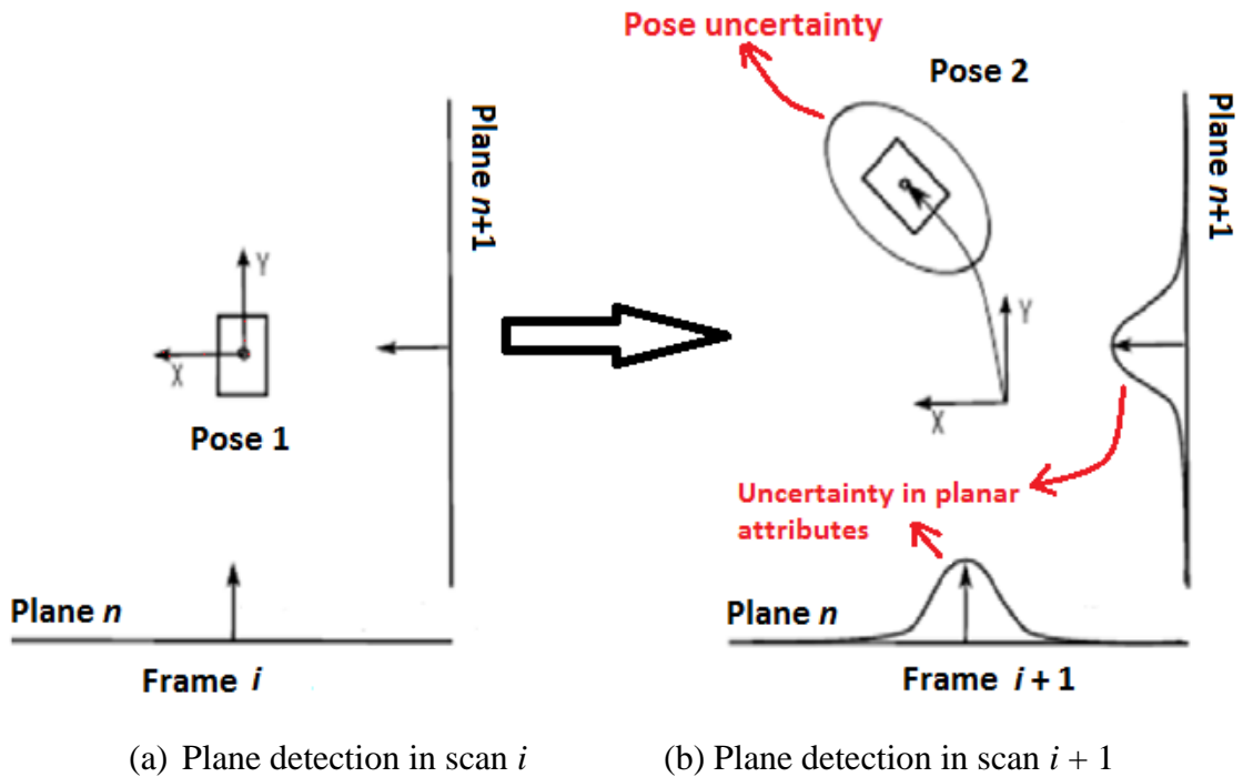
Fig. 3.2: Simplified 2D scan registration using plane uncertainty. (a) Initial pose of the robot in frame i with two planes detected and (b) Pose of the robot in the next frame.
