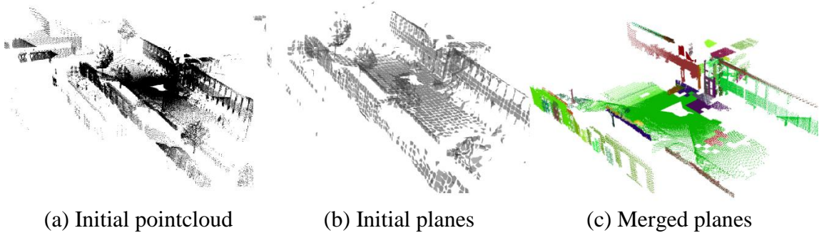
Figure 2.4: Segmentation procedure for the 1 st scan of the Freiburg campus data set. (a) initial pointcloud, (b) planes after initialization, (c) final planes
