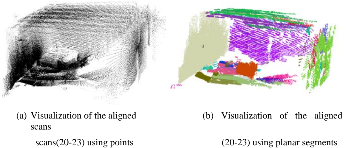
Figure 3.16: Resulted alignment of scans 20-23. Visualization using points (a) and using points of the planar segments (b)
