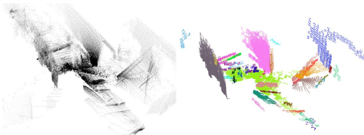
(a) Visualization of the aligned scans(70-72) using planar segments (b) Visualization of the scans(70-72) using points
