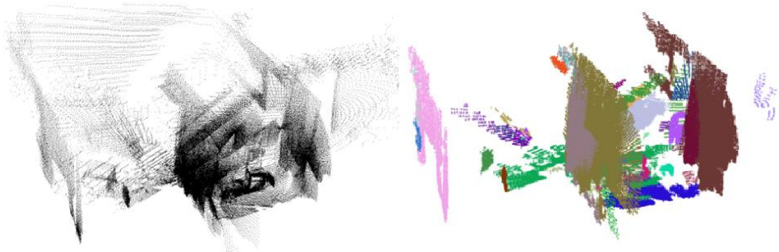
(c) Visualization of the aligned scans(86-89) using points aligned scans(86-89) using planar segments
