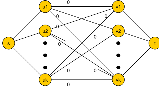
Figure 15.1: A simplified network. All edges adjacent to s or t have affine latency functions while all other edges, the internal edges, have zero latency
