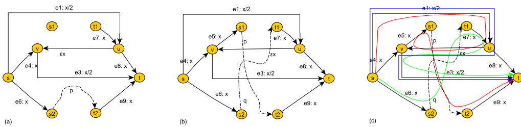
Figure 11.2: Possible subnetworks of G when there is no pair of vertex-disjoint paths connecting s_1 to t_1 and s_2 to t_2 . The subnetwork (a) contains an s_2 - t_2 path and does not include e_5 . In the subnetwork (b), we essentially have all edges of G . In (c), we depict a Nash flow that consists of three paths, each carrying r/3 units of flow, and has a bottleneck cost of r/3 .
