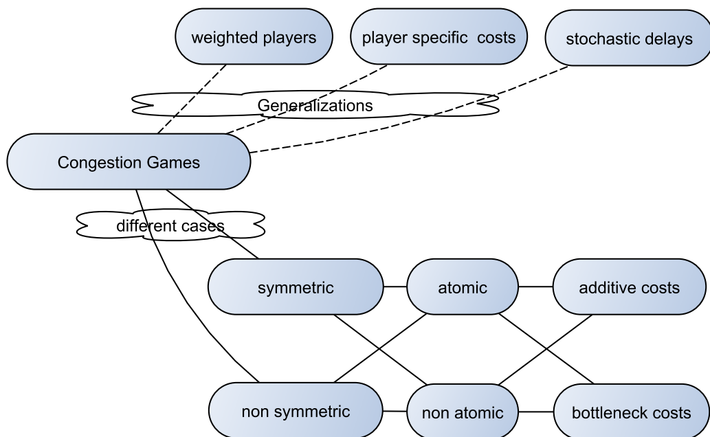
Figure 8.1: Network Congestion Games (small) map. The upper part captures the leading generalizations of CGs. The lower part captures the different cases arising by considering assumptions on the players' strategy spaces, on the players' types and on the players' strategies' costs.
