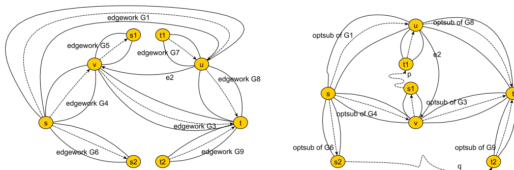
Figure 11.3: (a) The network G' constructed in the proof of Lemma 11.4. The structure of G' is similar to the structure of the network G in Fig. 11.1, with each external edge e_i , except for e_2 , replaced by the edgework G_i . (b) The structure of a best subnetwork H of G' , with \text{PoA} = 1 , when D contains a pair of vertex-disjoint paths, p and q , connecting s_1 to t_1 and s_2 to t_2 . To complete H , we use an optimal subnetwork (or simply, subedgework) of each edgework G_i .
