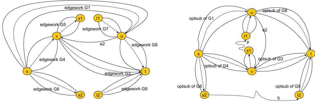
Figure 4.3: (a) The network G' constructed in the proof of Lemma 11.4. The structure of G' is similar to the structure of the network G in Fig. 11.1, with each external edge e_i , except for e_2 , replaced by the edgework G_i . (b) The structure of a best subnetwork H of G' , with \text{PoA} = 1 , when D contains a pair of vertex-disjoint paths, p and q , connecting s_1 to t_1 and s_2 to t_2 . To complete H , we use an optimal subnetwork (or simply, subedgework) of each edgework G_i .
