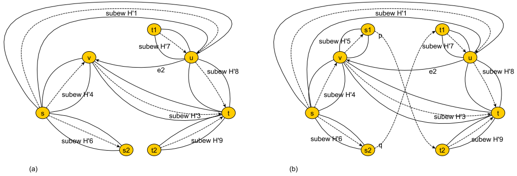
Figure 11.4: The structure of possible subnetworks of G' when there is no pair of vertex-disjoint paths connecting s_1 to t_1 and s_2 to t_2 . The subnetwork (a) contains a path outgoing from s_2 to either t_1 or t_2 , and no path outgoing from s_1 to either t_1 or t_2 . Hence, no flow can be routed through the edgework G_5 , and thus we can regard G_5 as being absent from H' . The subnetwork (b) essentially corresponds to the case where all edges of G' are present in H' .
