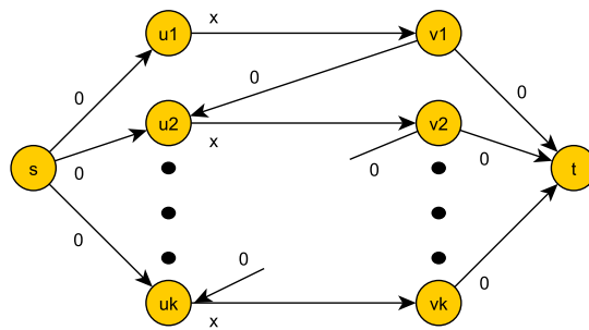
Figure 15.2: A network with \Theta(n) PoA. Optimally all the flow is splitted equally to the k direct paths while a bad Nash flow routes the traffic through path s - u_1 - v_1 - u_2 - v_2 - \dots - u_k - v_k - t
