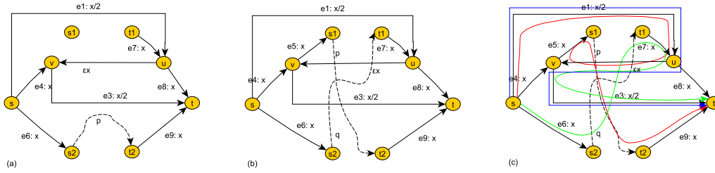
Figure 4.2: Possible subnetworks of G when there is no pair of vertex-disjoint paths connecting s_1 to t_1 and s_2 to t_2 . The subnetwork (a) contains an s_2 - t_2 path and does not include e_5 . In the subnetwork (b), we essentially have all edges of G . In (c), we depict a Nash flow that consists of three paths, each carrying r/3 units of flow, and has a bottleneck cost of r/3 .
