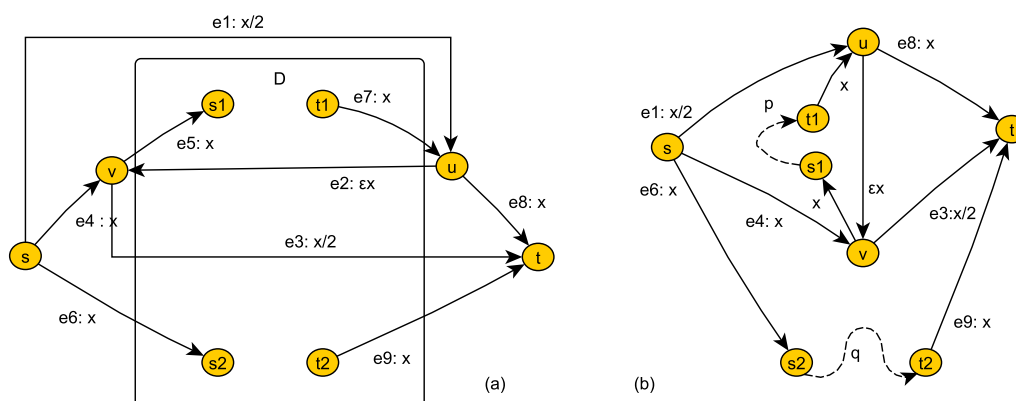
Figure 11.1: (a) The network G constructed in the proof of Lemma 11.1. (b) The best subnetwork of G , with \text{PoA} = 1 , for the case where D contains a pair of vertex-disjoint paths connecting s_1 to t_1 and s_2 to t_2 .
