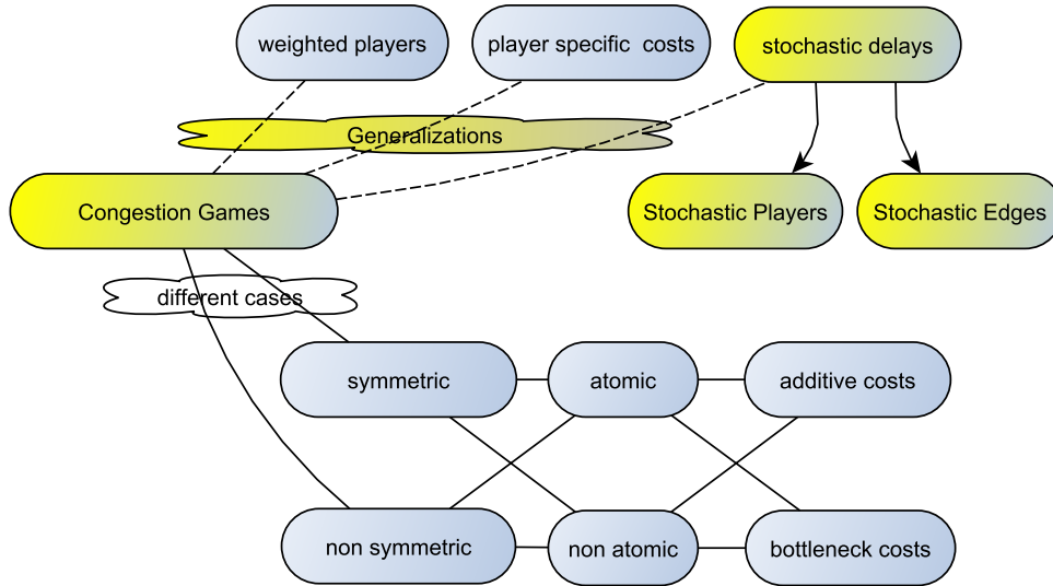
Figure 9.3: The introduced models and their positioning on the map.
