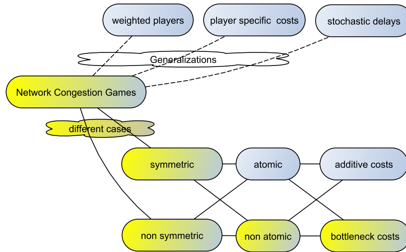
Figure 9.1: The main results (hardness results) of our work apply to both symmetric and asymmetric non atomic bottleneck costs games.
