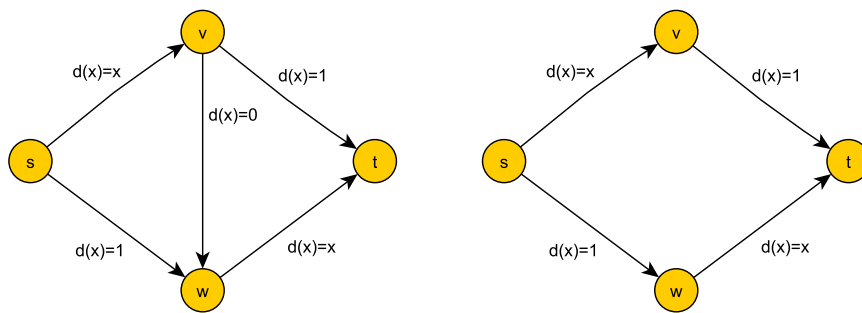
Figure 8.2: A unit of flow is to be routed from s to t . (a). The optimal (additive costs) flow routes 1/2 unit of traffic on the upper path (s, v, t) and 1/2 unit on the lower path (s, w, t) , and achieves a total latency of 3/2 . In the Nash flow, all traffic goes through the path (s, v, w, t) . The players' latency is 2, and the PoA is 4/3 . (b). Without the edge (v, w) , the Nash flow coincides with the optimal flow.
