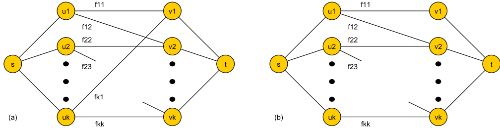
Figure 12.2: In (a), we have a cycle C = (u_1, v_2, u_2, \dots, v_k, u_k, v_1, u_1) in the intermediate subnetwork H_1[\Gamma(s) \cup \Gamma(t)] . We assume that f_{k1} is the minimum amount of flow through an edge of C in the equilibrium flow f . In (b), we have removed the edge e_{k1} , and show the corresponding change in the amount of flow on the remaining edges of C . Since the latency functions of the edges in C are constant, the change in the flow does not affect equilibrium.
