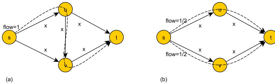
Figure 8.3: An example of Braess's paradox for bottleneck routing games. We consider a routing instance with identity latency functions and a unit of traffic to be routed from s to t . The worst Nash flow, in (a), routes all flow through the path (s, u, v, t) , and has a bottleneck cost of 1. On the other hand, the optimal flow routes 1/2 unit through the path (s, u, t) and 1/2 unit through the path (s, v, t) , and has a bottleneck cost of 1/2 . Hence, \text{PoA} = 2 . In the subnetwork (b), obtained by removing the edge (u, v) , we have a unique Nash flow that coincides with the optimal flow, and thus the PoA becomes 1.
