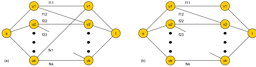
Figure 5.2: In (a), we have a cycle C = (u_1, v_2, u_2, \dots, v_k, u_k, v_1, u_1) in the intermediate subnetwork H_1[\Gamma(s) \cup \Gamma(t)] . We assume that f_{kl} is the minimum amount flow through an edge of C in the equilibrium flow f . In (b), we have removed the edge e_{kl} , and show the corresponding change in the amount of flow on the remaining edges of C . Since the latency functions of the edges in C are constant, the change in the flow does not affect equilibrium.
