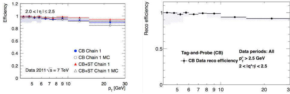
Figure 3.6: Comparison of muon reconstruction efficiencies as a function of p_T , using data collected during 2011 (left) and 2012 (right).
