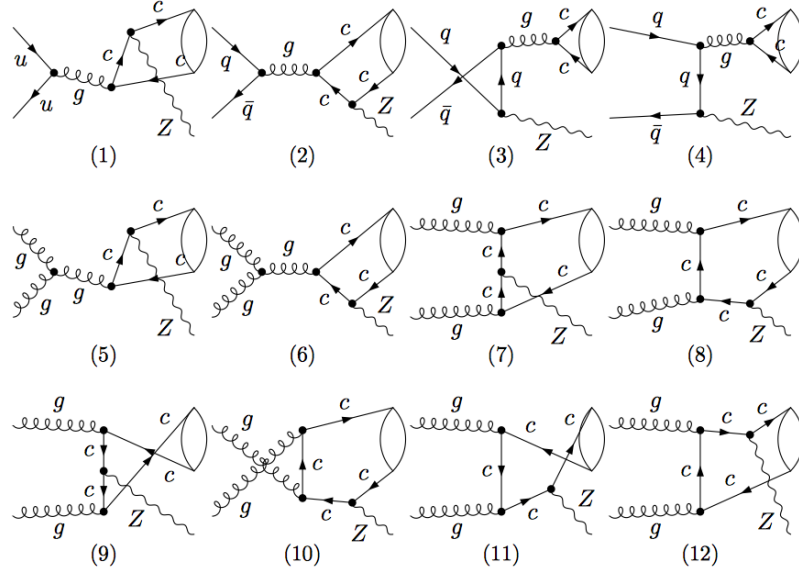
Figure 1.3: Tree-level Feynman diagrams for the production of prompt J/\psi + Z . Diagrams 1 – 4 show the diagrams with q\bar{q} initial state and 5 – 12 with gg .
