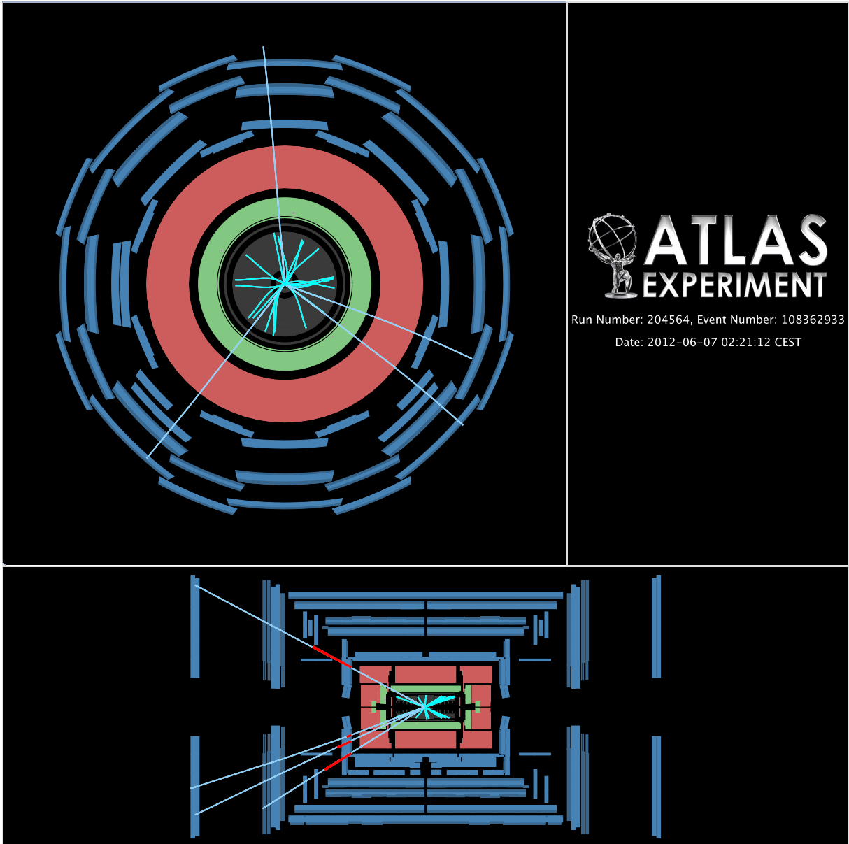
Figure 4.6: The main event display for event 108362933 in run 204564. Z muons have p_{\text{T}}^{\mu_1} = 60 \text{ GeV} , p_{\text{T}}^{\mu_2} = 17 \text{ GeV} and \eta^{\mu_1} = -0.4 , \eta^{\mu_2} = -2.2 ( \mu_1 pointing at 1 o'clock and \mu_2 at 8 o'clock). J/\psi muons have p_{\text{T}}^{\mu_3} = 7 \text{ GeV} , p_{\text{T}}^{\mu_4} = 7 \text{ GeV} and \eta^{\mu_3} = 1.8 , \eta^{\mu_4} = 1.4 ( \mu_3 pointing at 6 o'clock and \mu_4 at 6 o'clock). The invariant mass of the Z boson candidate is found to be 85.0 GeV and J/\psi 3.1 GeV.
