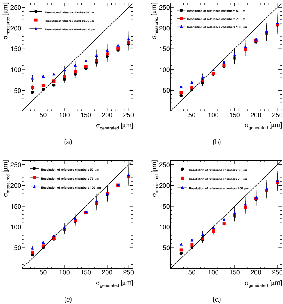
Figure 6.8: (a) Comparison of measured and generated resolution, assuming three different scenarios. With the black circles the reference detectors are modelled to have 50 \mu\text{m} resolution, with red squares 75 \mu\text{m} resolution and with blue triangles 100 \mu\text{m} resolution. The black line assumes that the generated value is equal to the measured. (b), (c), (d) Same as Figure 6.8(a), but the test chamber positioned in the alternative positions (b), (c) and (d), respectively (see Figure 6.6). The errors on all figures are multiplied by 10 in order to be visible.
