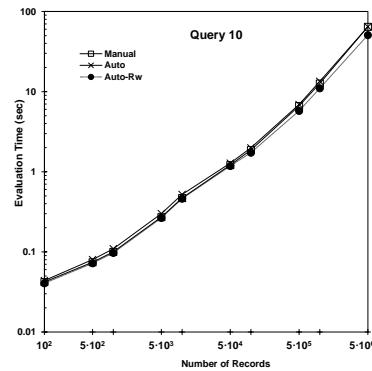
(χ) Query 10
