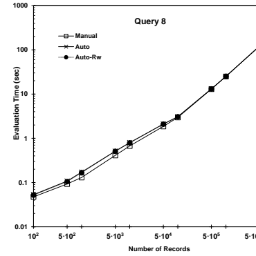
(η) Query 8
