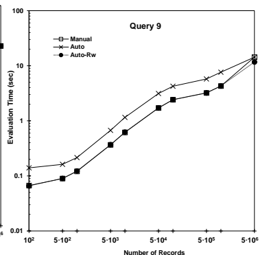
(ι) Query 9
