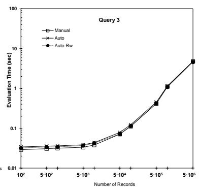
(ς) Query 3
