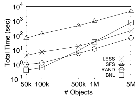
(β') Independent
