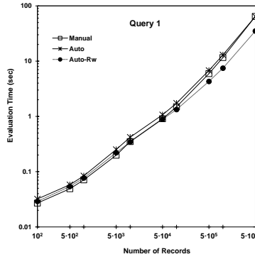
(α) Query 1
