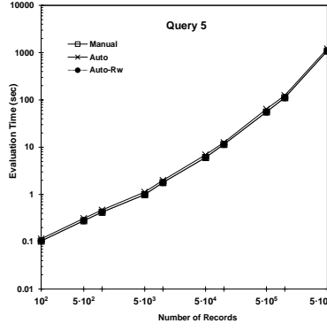
(ε) Query 5
