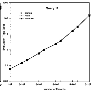
(λ) Query 11
