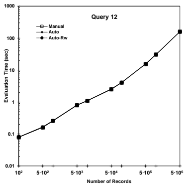
(μ) Query 12
