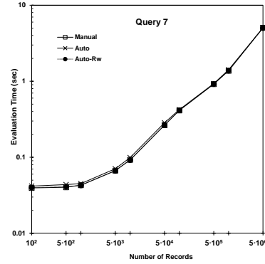
(γ) Query 7
