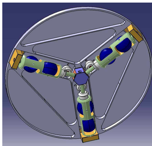
Fig 2.4 Layout of the three axles (CAD design) ROMNI robot [Mour06]
