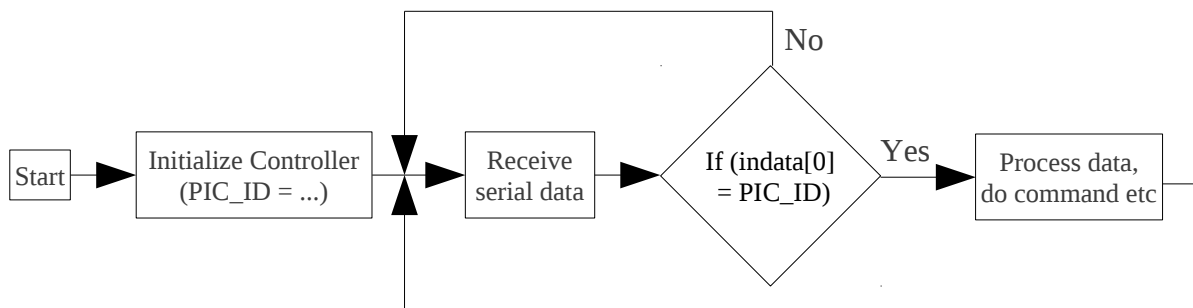
Fig 6.3 Wheel's Micro-controller PIC program algorithm using XBee
