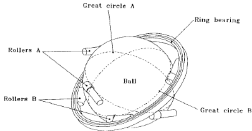
Fig 2.5 Spherical ball wheel [West95]
