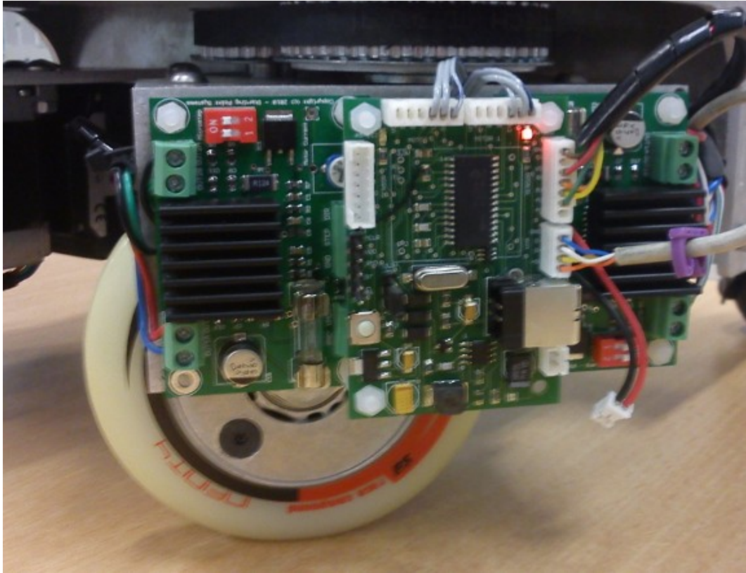
Fig 5.8 Other Caster Wheel Assembly
