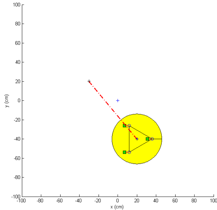
Fig 4.3 Robot's snapshot at t=0s
