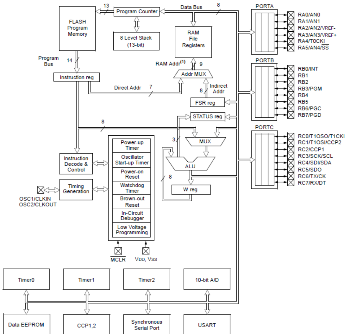
Fig 2.6 16F87X PIC Architecture [Pekm09]
