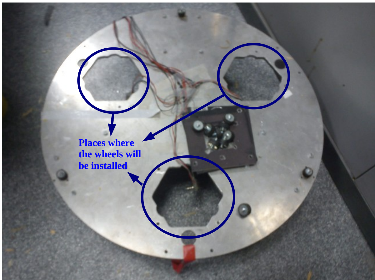
Fig 7.1 1 st Robot's Chassis
