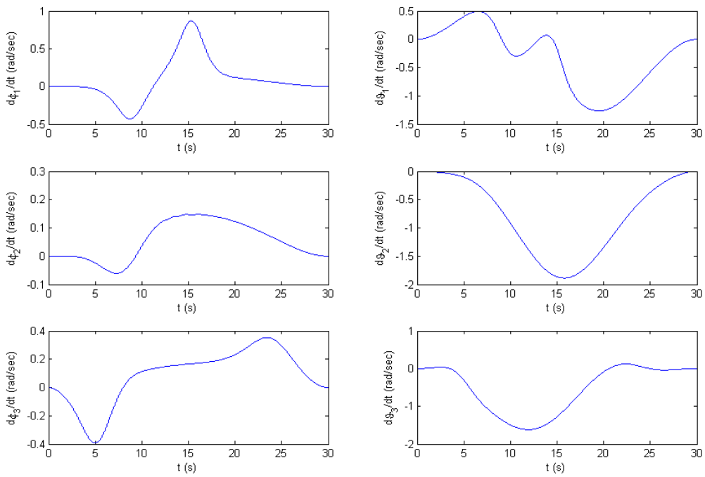
Fig 4.8 Joint Velocities
