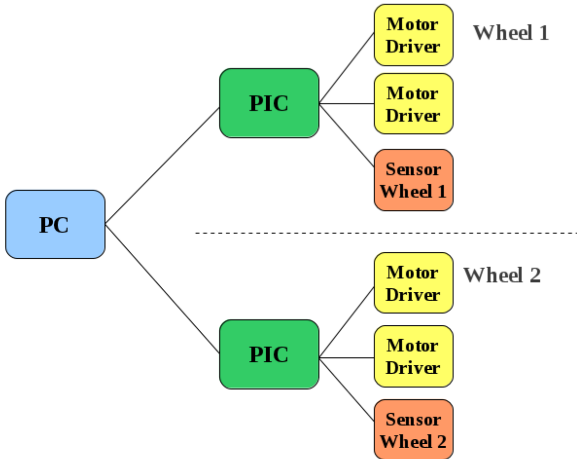
Fig 6.2 Connectivity configuration 2
