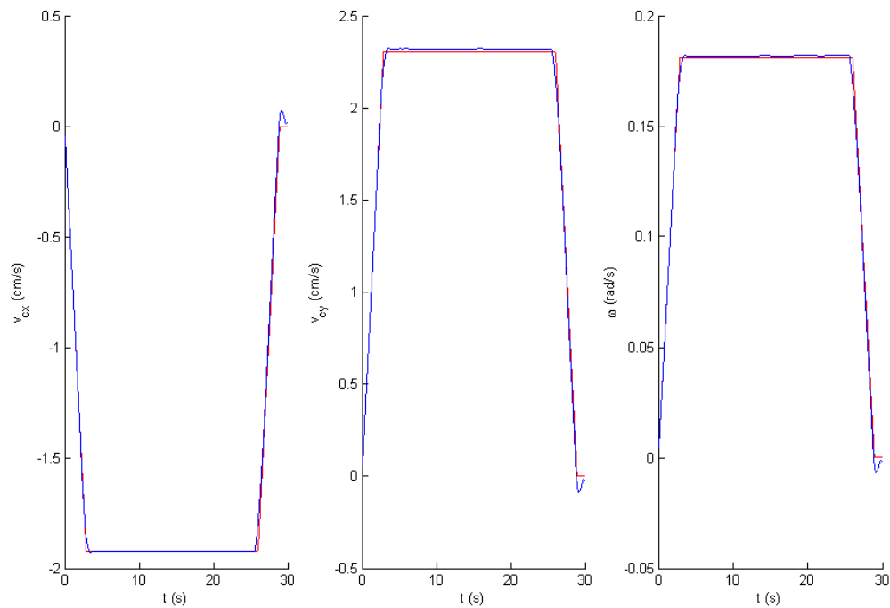
Fig 4.23 Robot's Velocities
