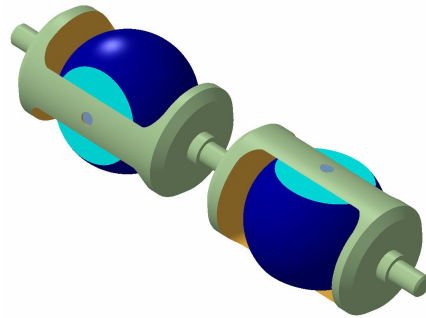
Fig 2.2 Spherical Orthogonal Wheel [Mour06]
