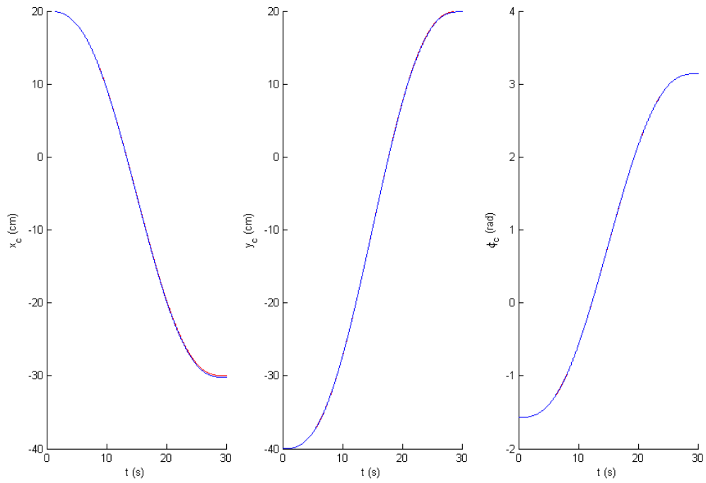
Fig 4.7 Robot's position
