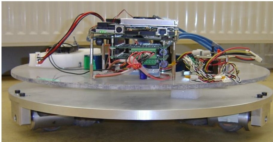
Fig 2.3 ROMNI robot [Mour06]
