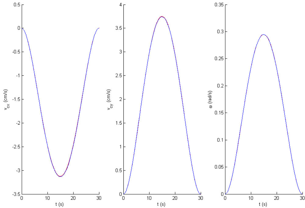
Fig 4.9 Robot's velocities
