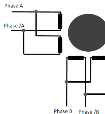
Fig 2.8 Two-Phase Bipolar motor [Sopr57] [Tech23]
