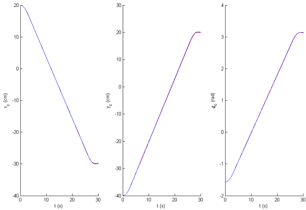
Fig 4.21 Robot's position
