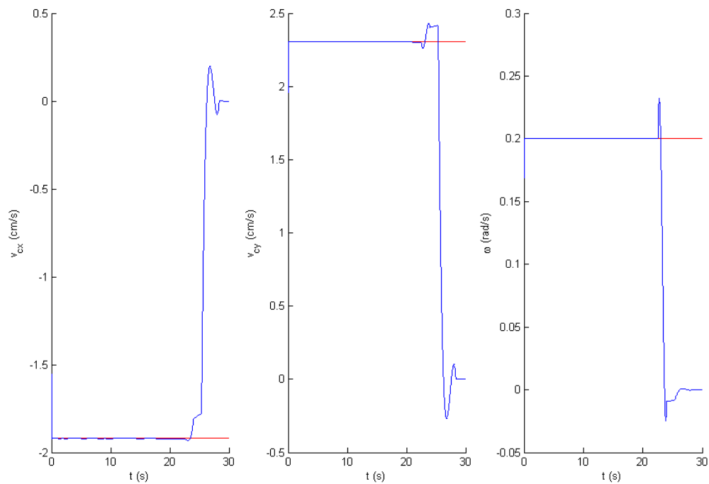
Fig 4.16 Robot's Velocities
