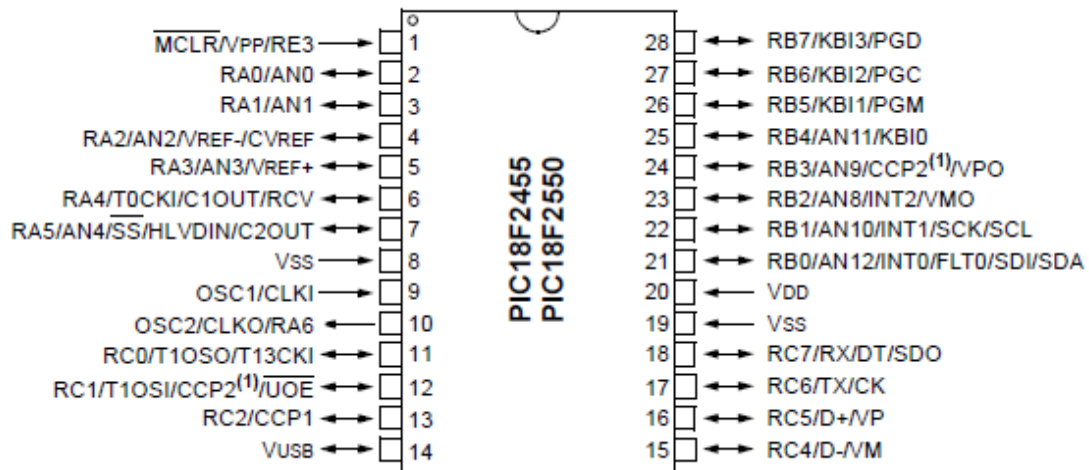
Fig 5.4 Micro-controller PIC pin diagram [PIC18]
