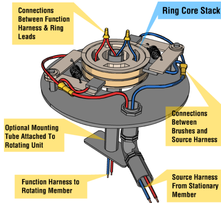
Fig 5.1 Slip Ring example
