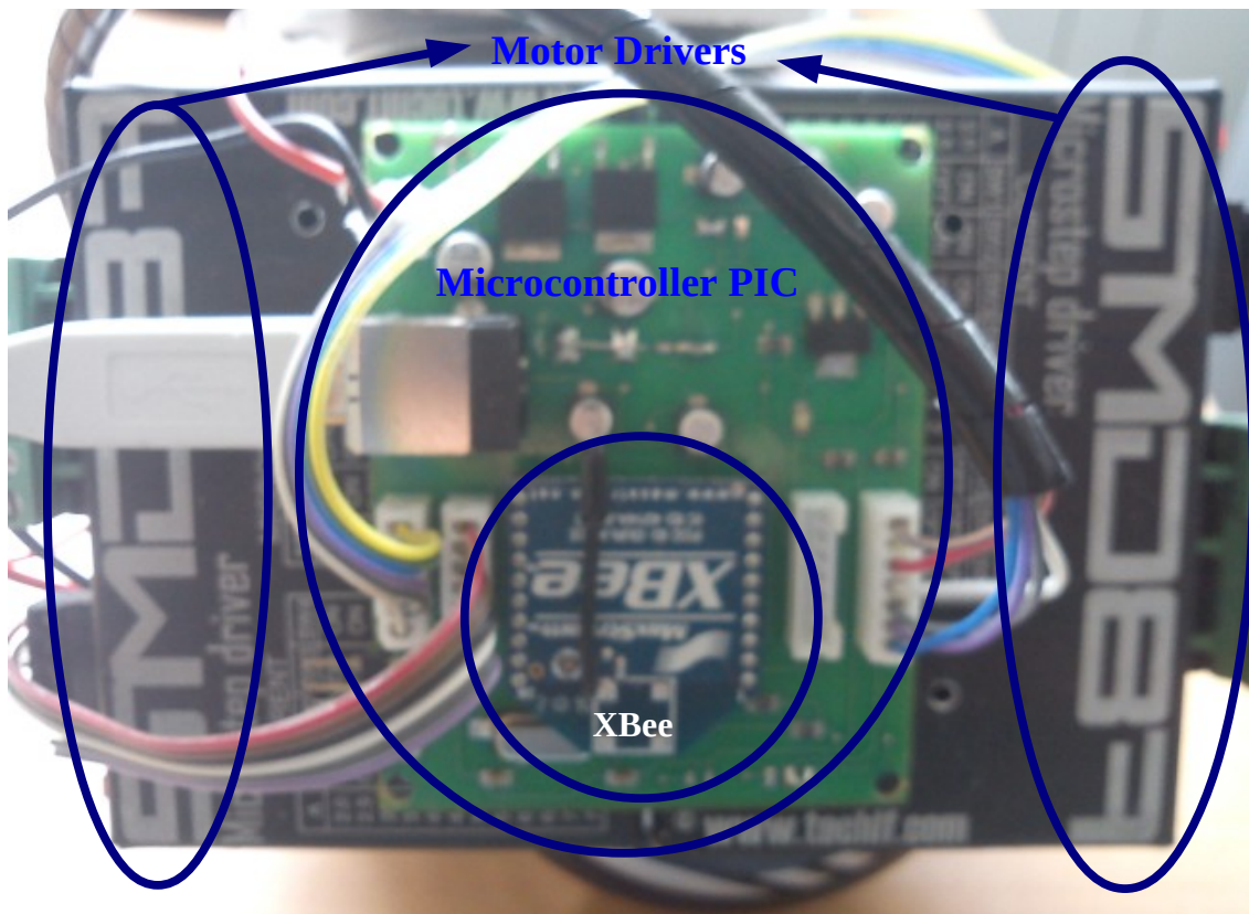
Fig 5.7 Electronics on the wheel
