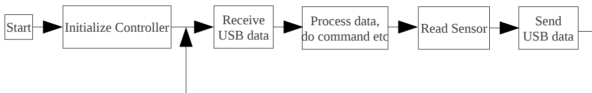
Fig 6.4 Wheel's Micro-controller PIC's program algorithm using USB
