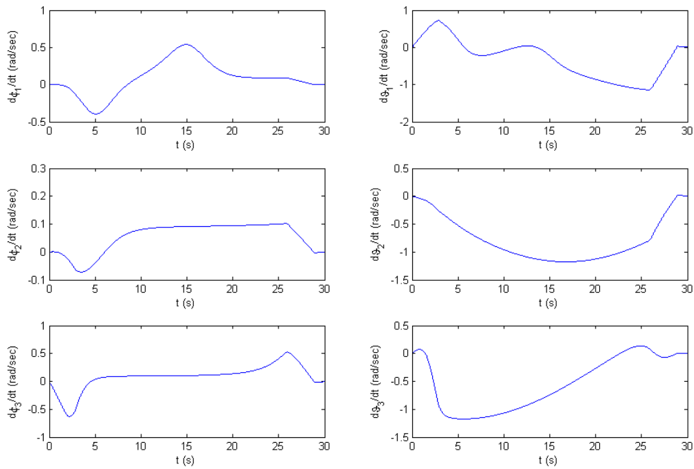
Fig 4.22 Joint Velocities
