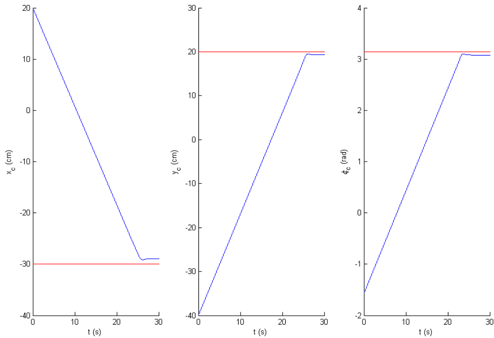
Fig 4.14 Robot's position
