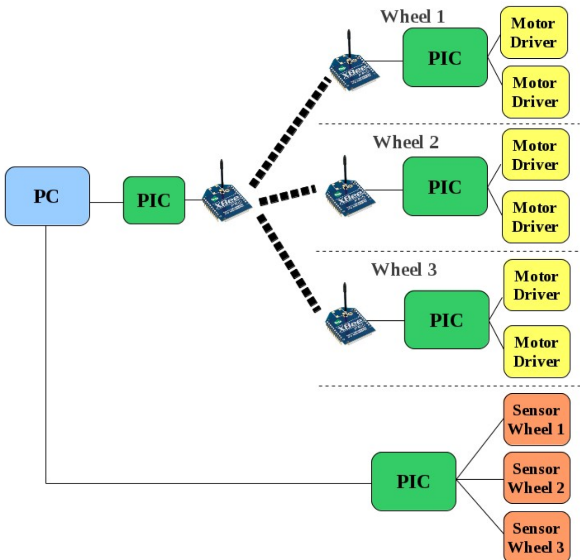
Fig 6.1 Connectivity configuration 1
