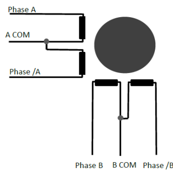
Fig 2.7 Two-Phase Unipolar stepper motor [Sopr57] [Tech23]
