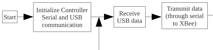
Fig 6.6 Computer's Micro-controller PIC program algorithm for XBee transmission
