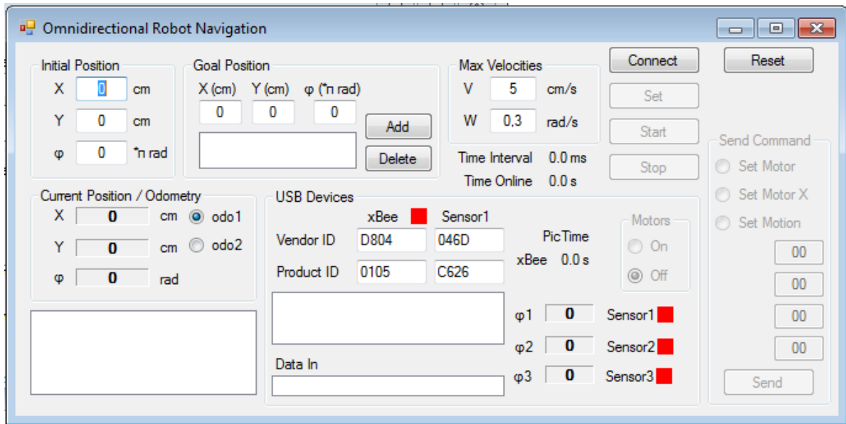
Fig 6.7 User Interface program
