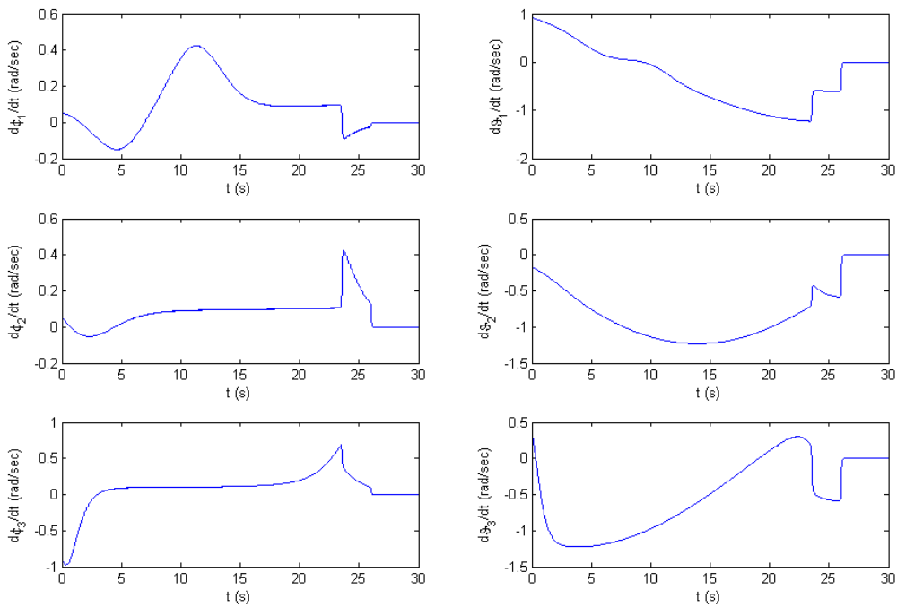
Fig 4.15 Joint Velocities
