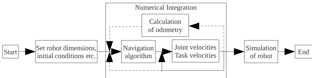
Fig 4.1 MatLAB simulation algorithm
