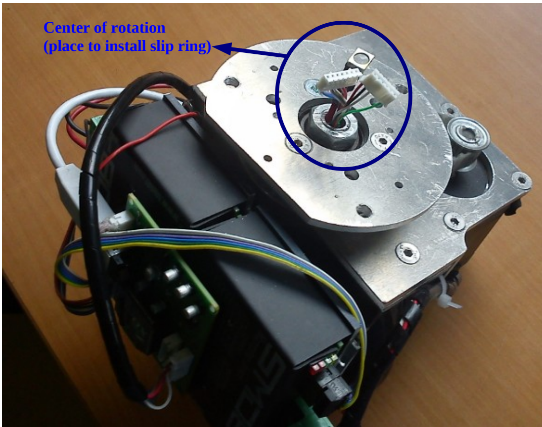
Fig 5.9 Top of caster wheel
