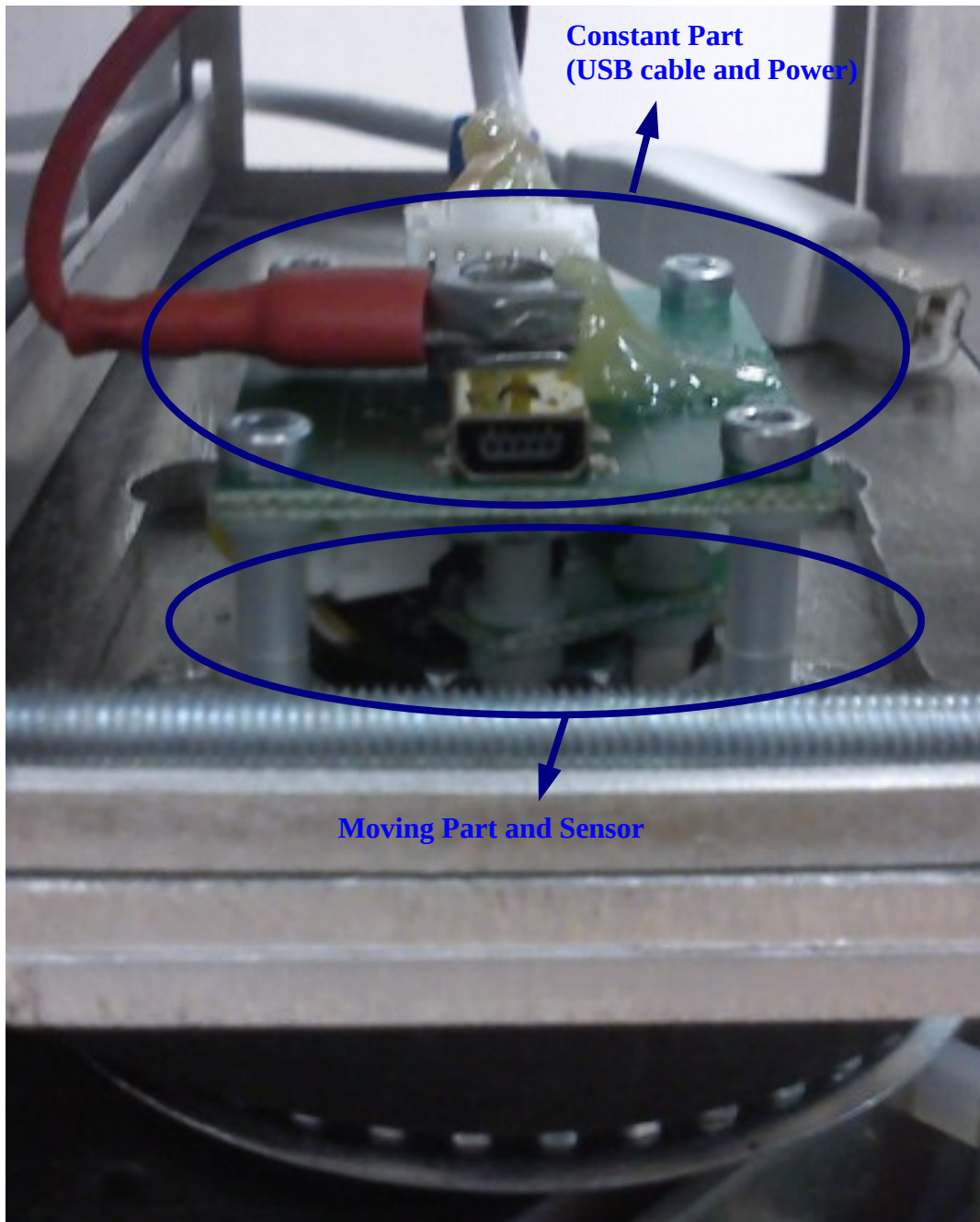
Fig 5.10 Slip Ring on robot
