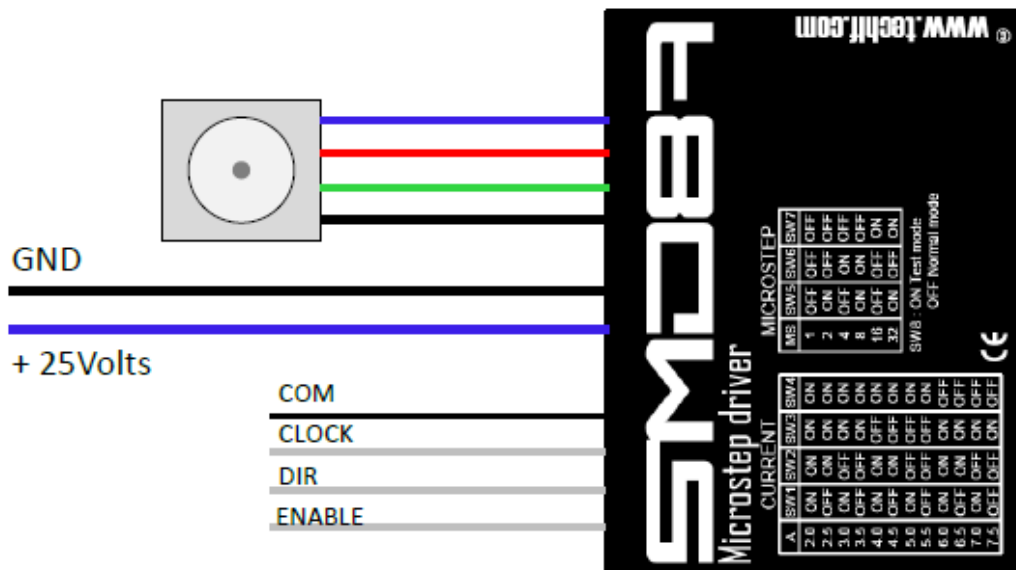
Fig 5.2 Microstep motor SMD8A pin diagram [Tech8A]
