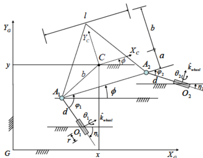
Fig 3.1 Geometrical representation of the robot [Lee05]
