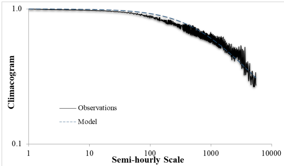
Fig.2.10: Climacogram for wave height.
