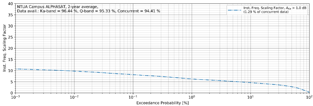
Figure 10-4: IFSF Exceedance Probability, Campus Ka-band ALPHASAT vs Q-band ALPHASAT
