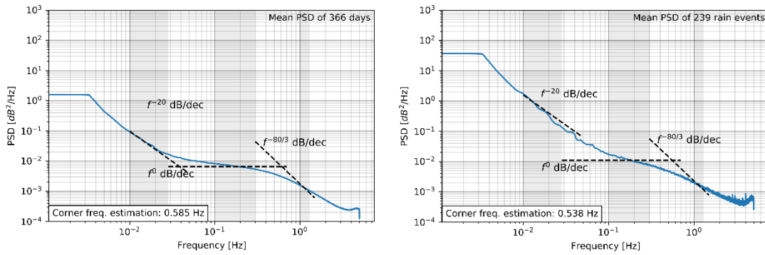
Figure 11-19: Yearly spectra for LTCP Ka-band ALPHASAT, 2019-2020
