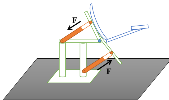
Figure 4-38: The push-pull gas spring architecture supporting the antenna
