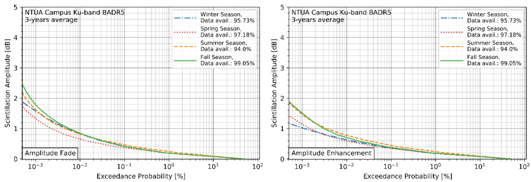
Figure 11-26: Seasonal scintillation amplitude fade & enhancement for Campus Ku-band BADR5
