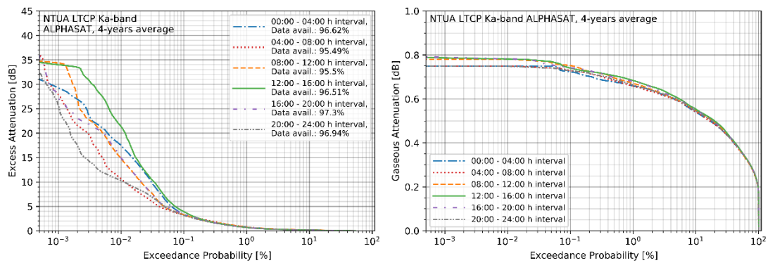
Figure 5-31: Diurnal attenuation probability (CCDF) for LTCP Ka-band ALPHASAT, Left: Excess Attenuation, Right: Gaseous Attenuation
