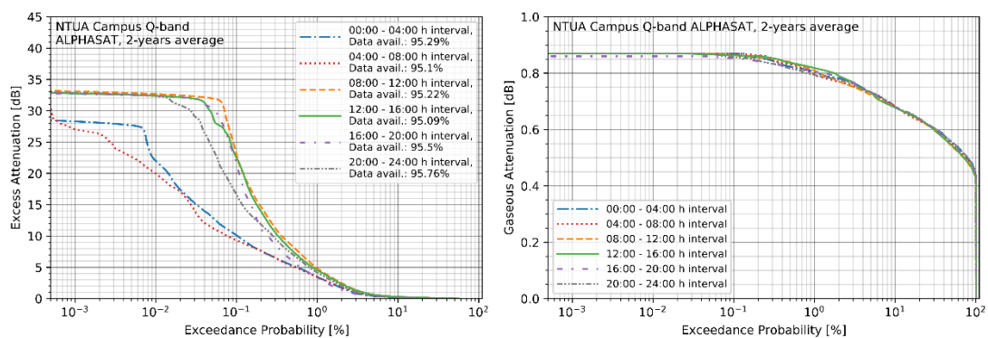
Figure 5-32: Diurnal attenuation probability (CCDF) for Campus Q-band ALPHASAT, Left: Excess Attenuation, Right: Gaseous Attenuation
