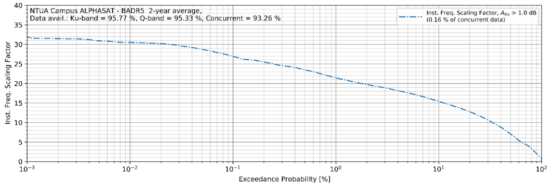
Figure 10-19: IFSF Exceedance Probability, Campus Ku-band BADR5 vs Q-band ALPHASAT
