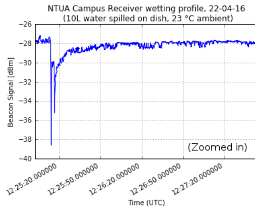
Figure 4-42: NTUA antenna wetting profile (zoomed in)
