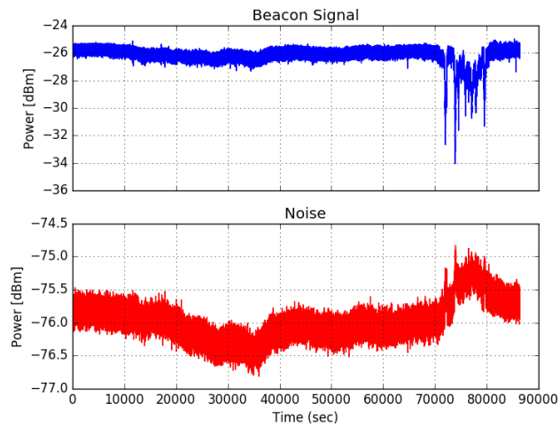
Figure 4-17: Actual beacon and noise power time series for a day involving a light rain event (13/06/2016) [9], © 2017 IEEE
