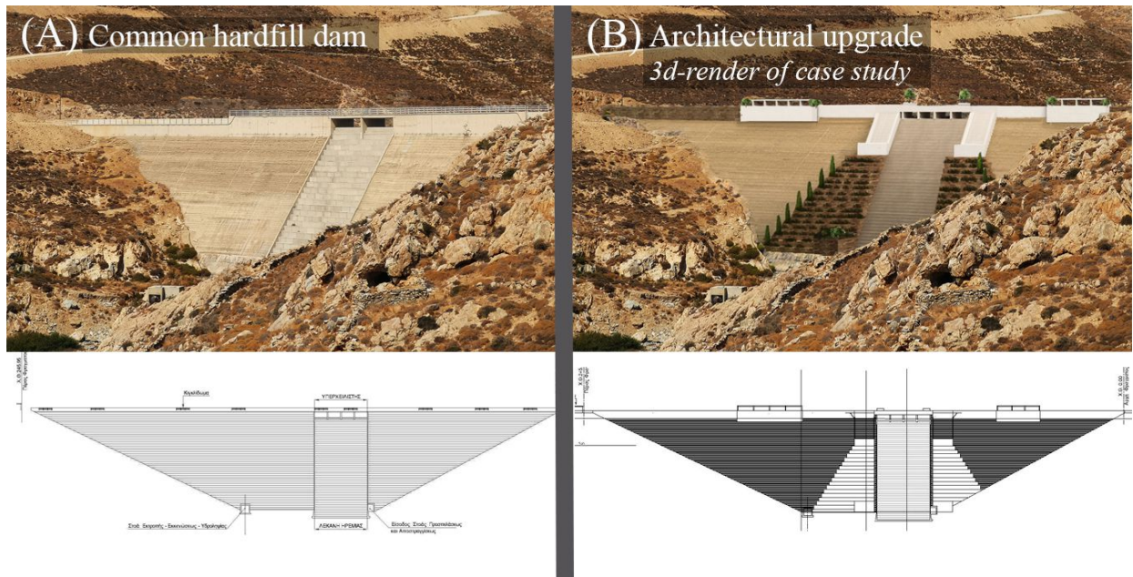
Figure 29. (A) left side: photograph of a hardfill dam (in Steno - Serifos, Greece) and common front view of a hardfill dam. (B) right side (case study): 3d render of the architectural design proposition and front view of the dam after the architectural upgrades.
