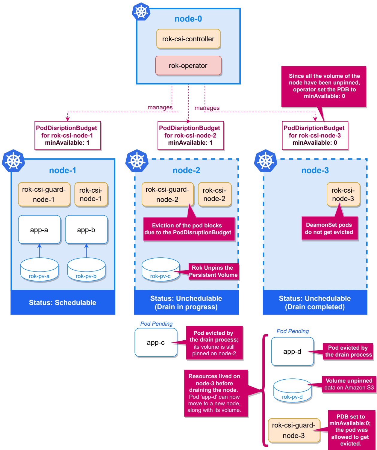
Figure 3.1: Protecting Local Data with Rok CSI Guard Pods
