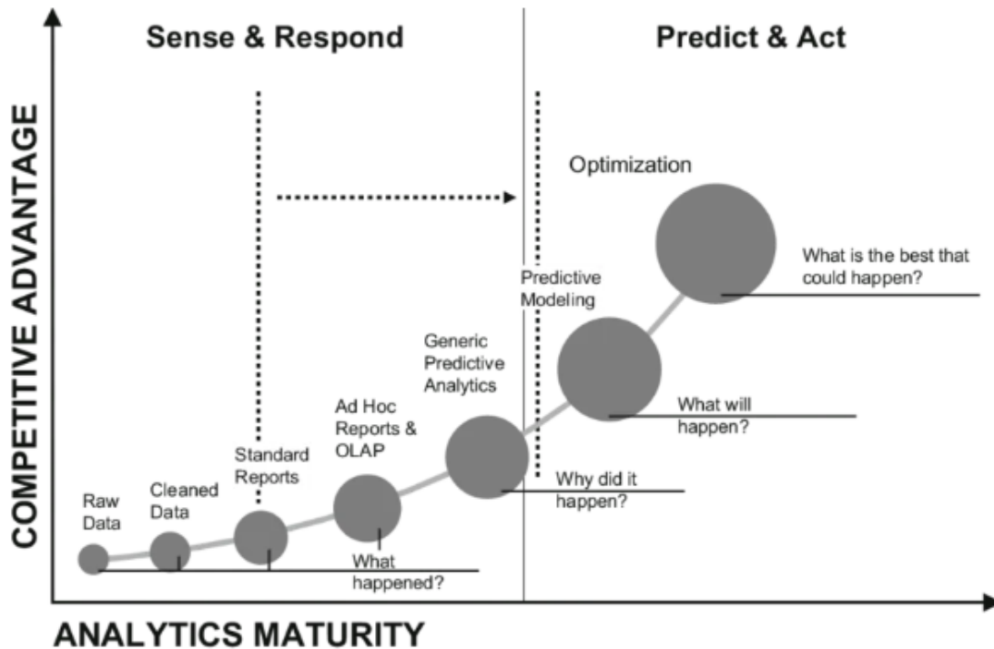
Figure 3.2. Analytics Stages [1]
