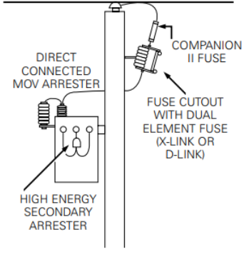
Figure 6. Lightning-protected transformer (LPT) installation
