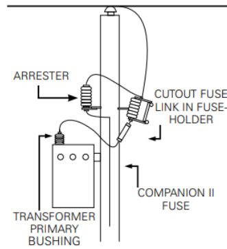
Figure 2. Load-side cutout installation
