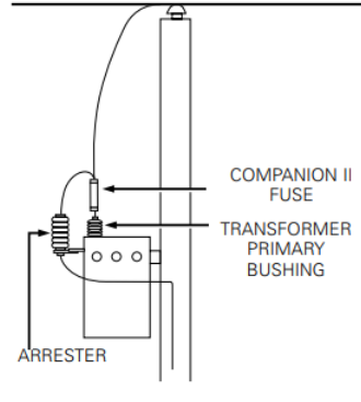
Figure 5. Completely self-protected (CSP) transformer installation
