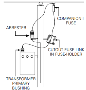
Figure 3. Hot-line/bail installation
