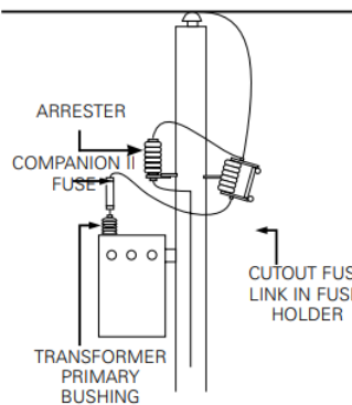
Figure 4. Bushing mount installation
