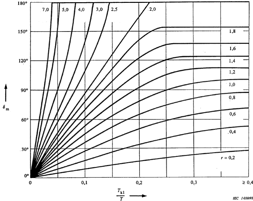
Figure 6 – Maximum swing out angle \delta_m for a given maximum short-circuit duration T_{k1}
