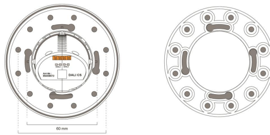
dimensions mounting ring
