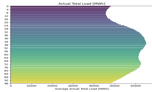
Figure 10: Germany: quarterly average Actual Total Load [MWh]
