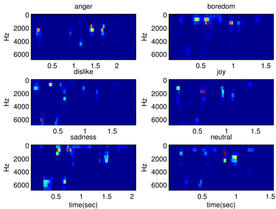
Mean Teager Energy –13 channels – speak11 – senta02
